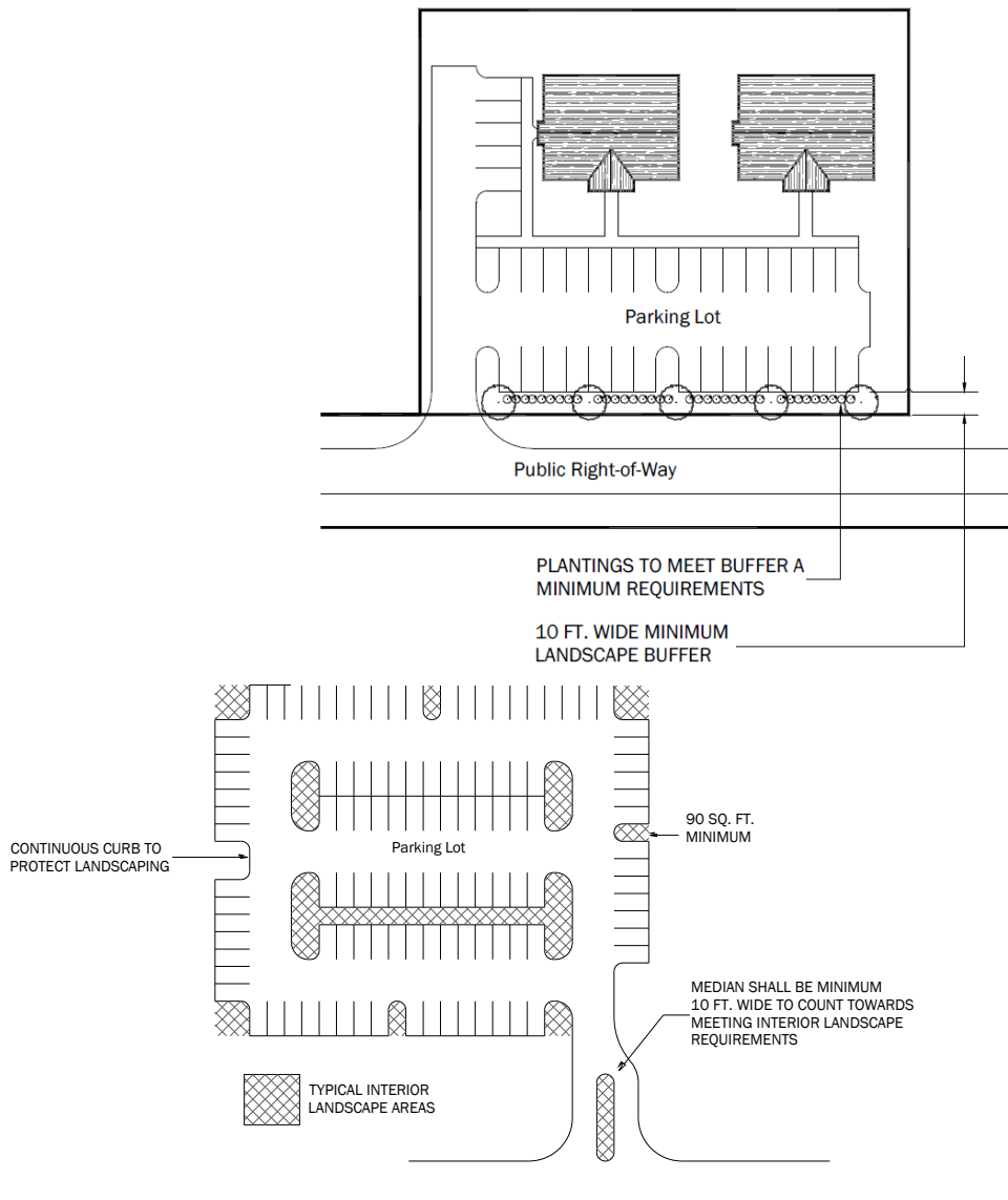
Figure 4.06.04.A: Illustration of Parking Lot Landscaping
